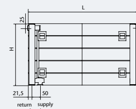
HP-V valve radiator Rear view
